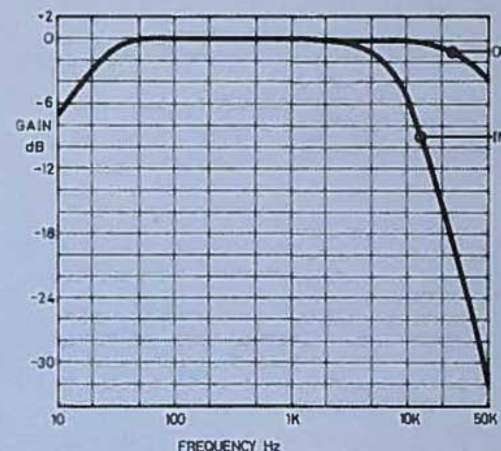
Rumble and High Filter Responses
