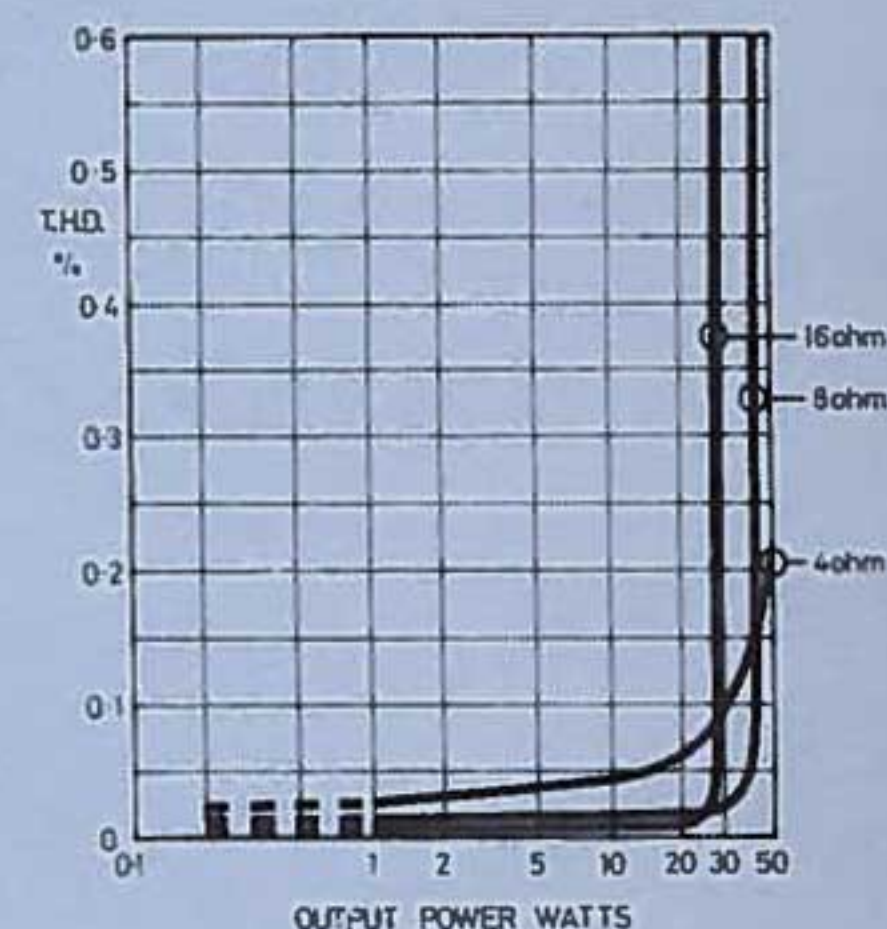
THD vs Power Output 1kHz
